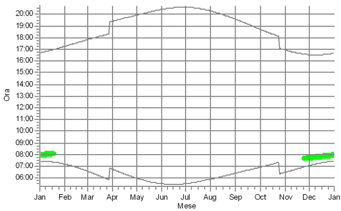
O: Shadow Receptor: 1,0 × 1,0 Azimuth: 0,0° Slope: 90,0° (16)
