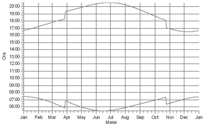
W: Shadow Receptor: 1,0 × 1,0 Azimuth: 0,0° Slope: 90,0° (24)
