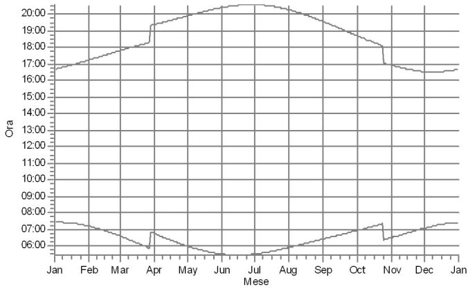
M: Shadow Receptor: 1,0 × 1,0 Azimuth: 0,0° Slope: 90,0° (14)
