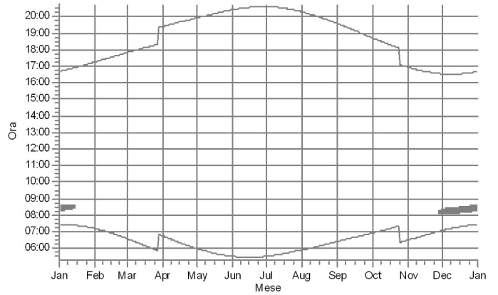
V: Shadow Receptor: 1,0 × 1,0 Azimuth: 0,0° Slope: 90,0° (23)
