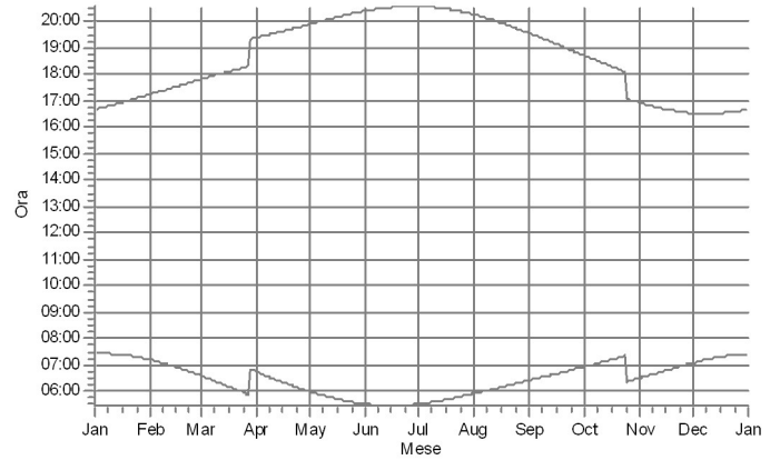
J: Shadow Receptor: 1,0 × 1,0 Azimuth: 0,0° Slope: 90,0° (11)
