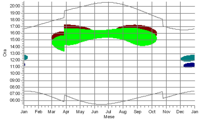
8: VESTAS V126-3.3 GridStreame 3300 126.0 !O!hub: 117,0 m (TOT: 180
