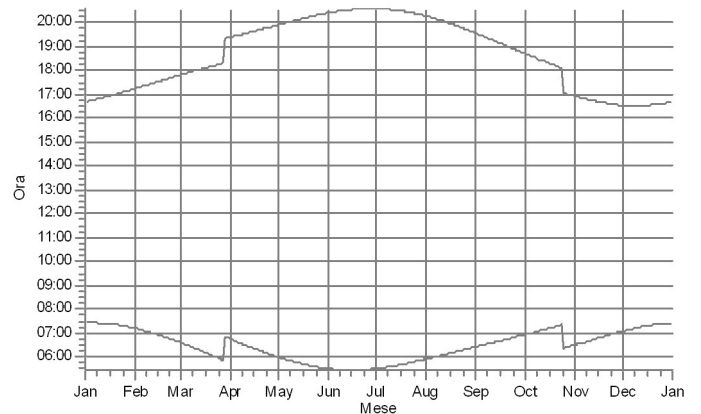
L: Shadow Receptor: 1,0 × 1,0 Azimuth: 0,0° Slope: 90,0° (13)
