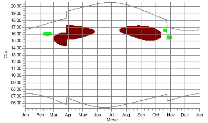
H: Shadow Receptor: 1,0 × 1,0 Azimuth: 0,0° Slope: 90,0° (9)
