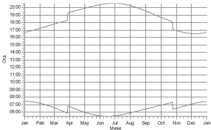
Q: Shadow Receptor: 1,0 × 1,0 Azimuth: 0,0° Slope: 90,0° (18)
