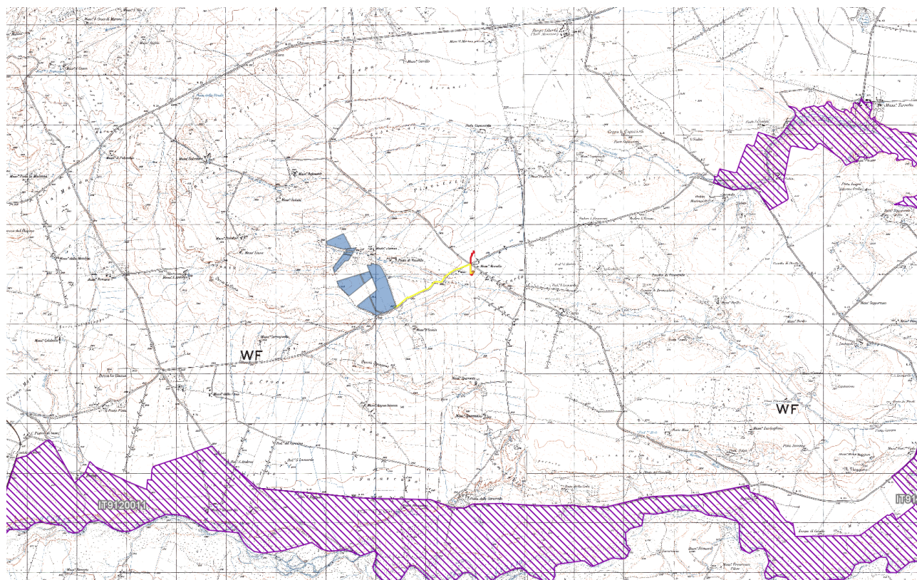
Fig. 2-4: Aree Natura 2000
