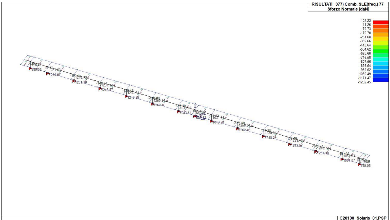
43_RIS_N_077_Comb. SLE(freq.) 77
