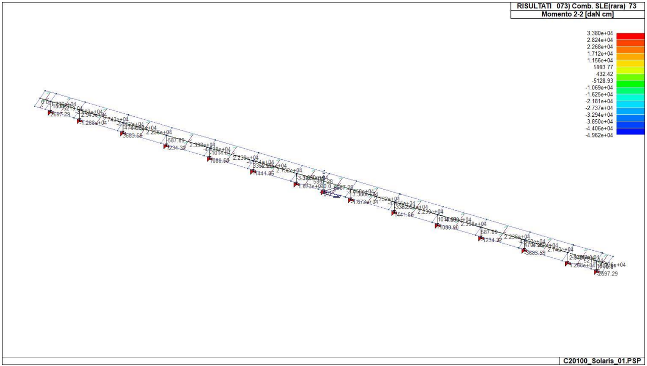
43_RIS_M2_073_Comb. SLE(rara) 73
