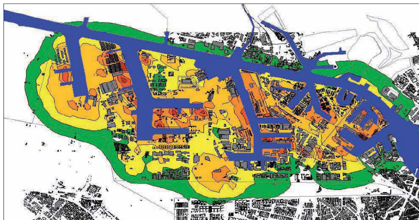
Mappa acustica Amsterdam (Fonte: Good Practice Guide on Port Area Noise Mapping and Management).
