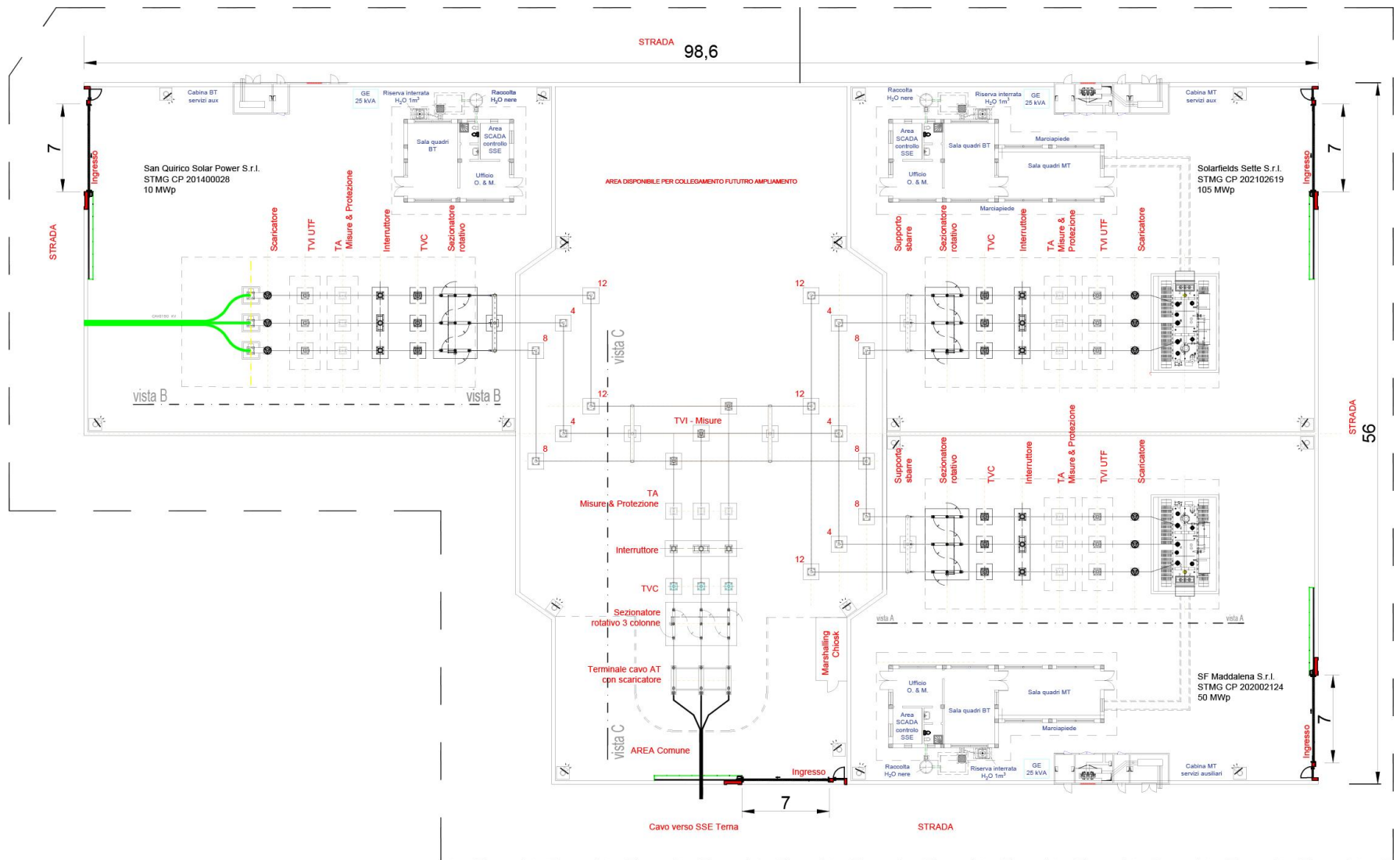
Figura1: Planimetria SS Terna
