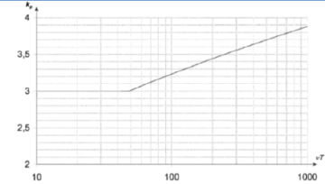
Figure 6.2 — Peak factor k_p = \sqrt{2 \cdot \ln(v \cdot T)} = \frac{0,6}{\sqrt{2 \cdot \ln(v \cdot T)}} or k_p = 3 whichever is larger
