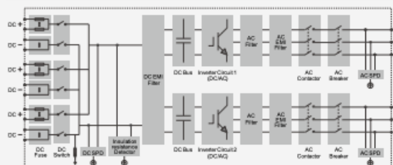
Circuit Diagram
