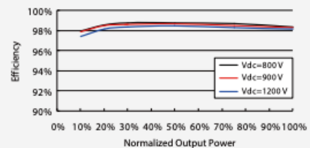
Efficiency Curve
