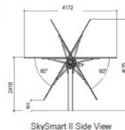
Fig. 9 – Datasheet tracker SkySmart II (ARCTECH)
