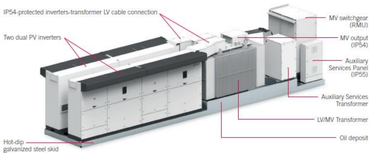
Figura 7-11 – Layout tipico Power Station
