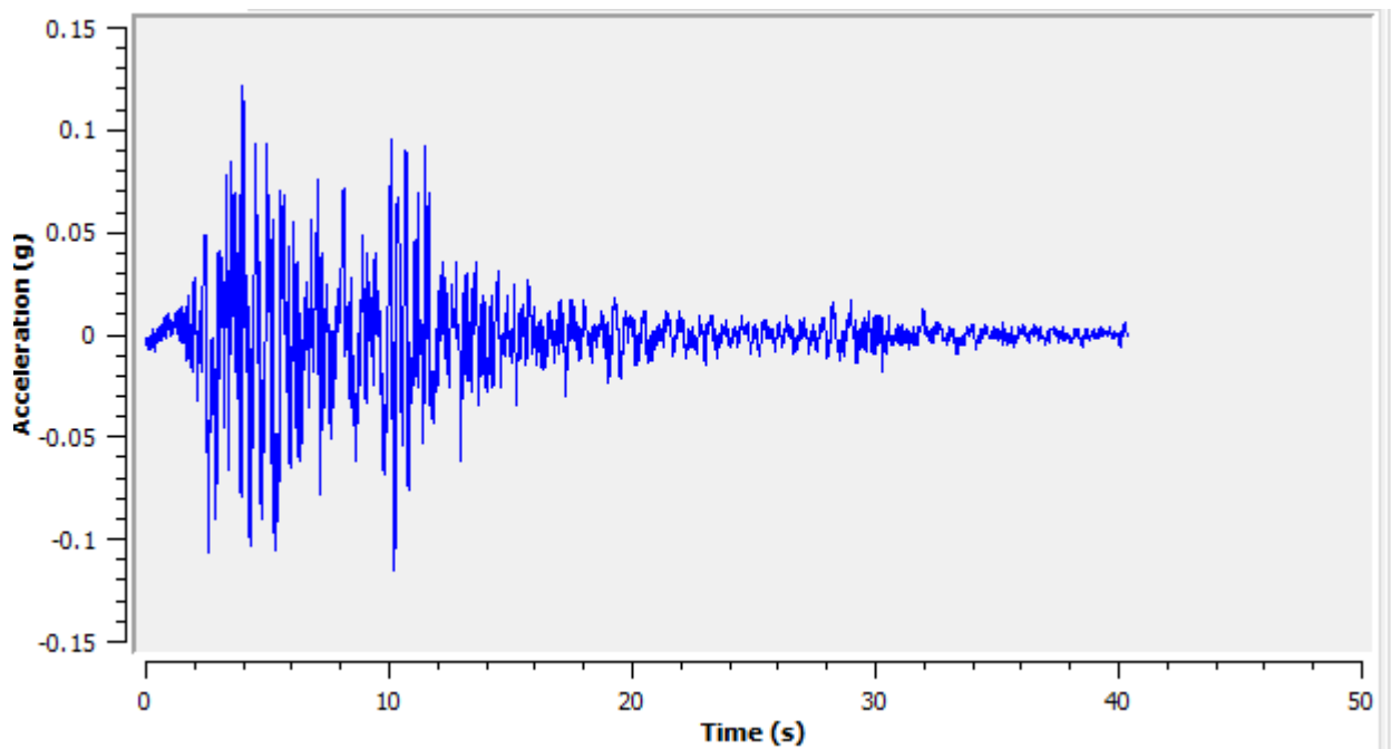
Figura 4: Accelerogramma 000198xa
