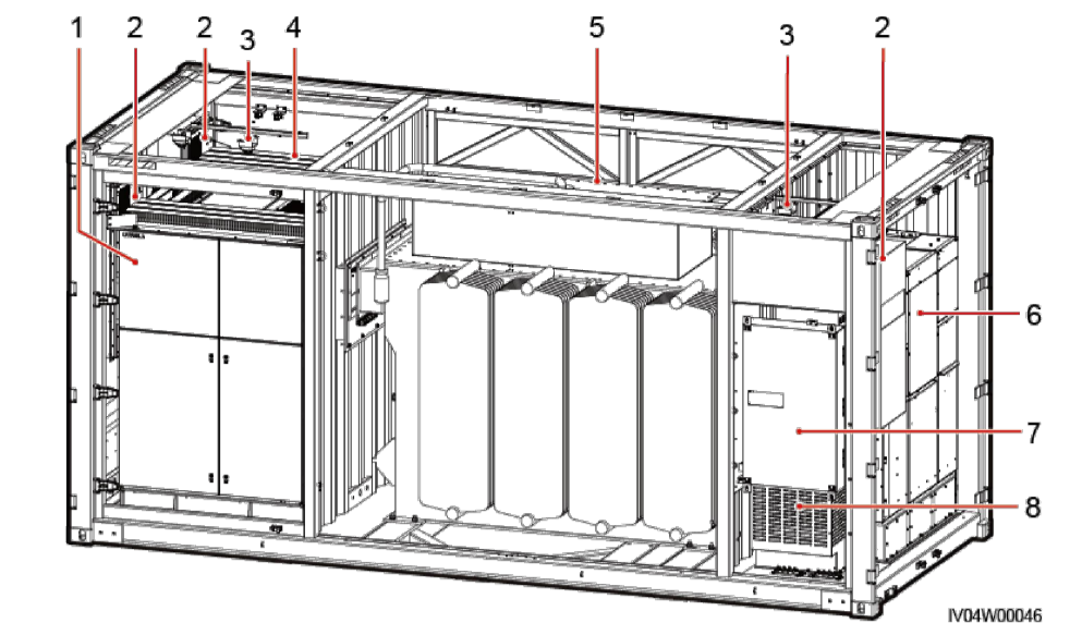
Figure 2-5 STS components
