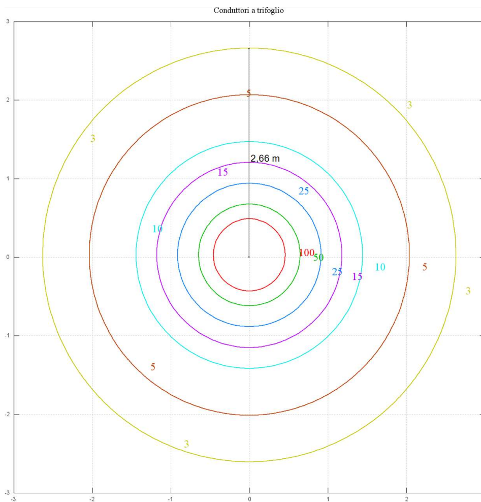
Figura 4. curve isolivello cavo AT
