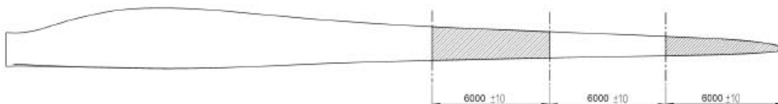
Hatched Area to be painted RAL2009
