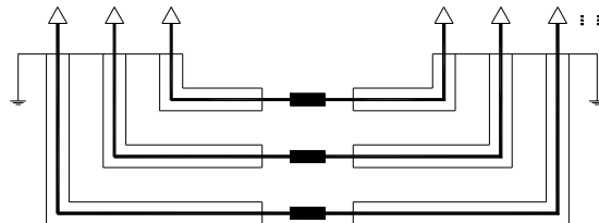
SINGLE POINT BONDING
