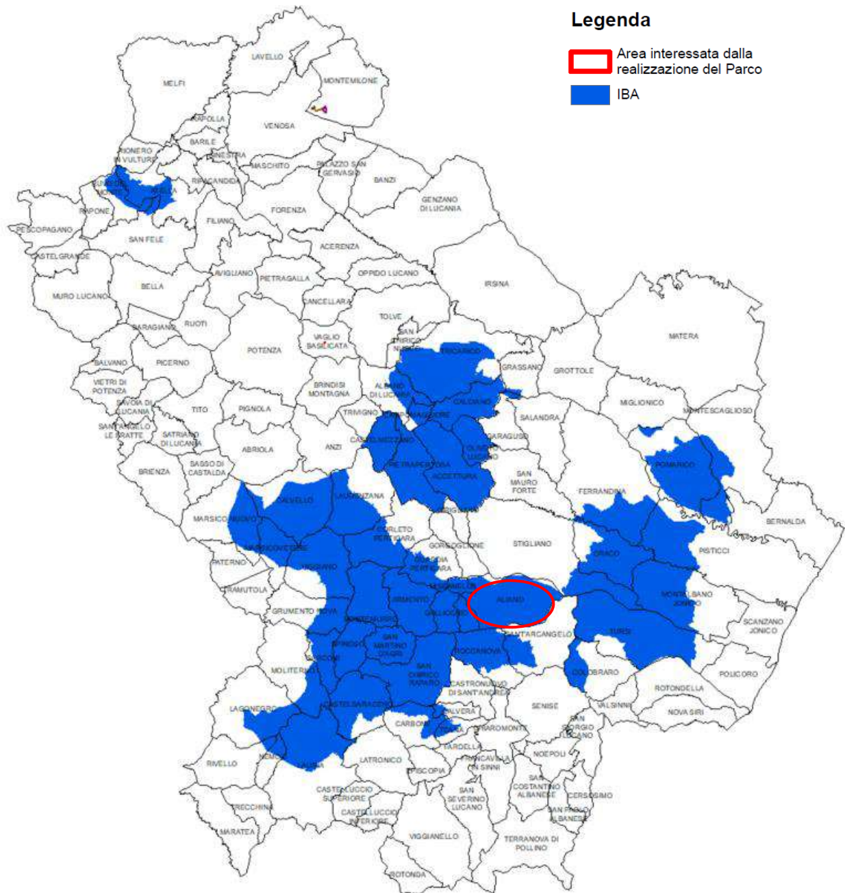
Figura 3.10. – AREE IBA.
