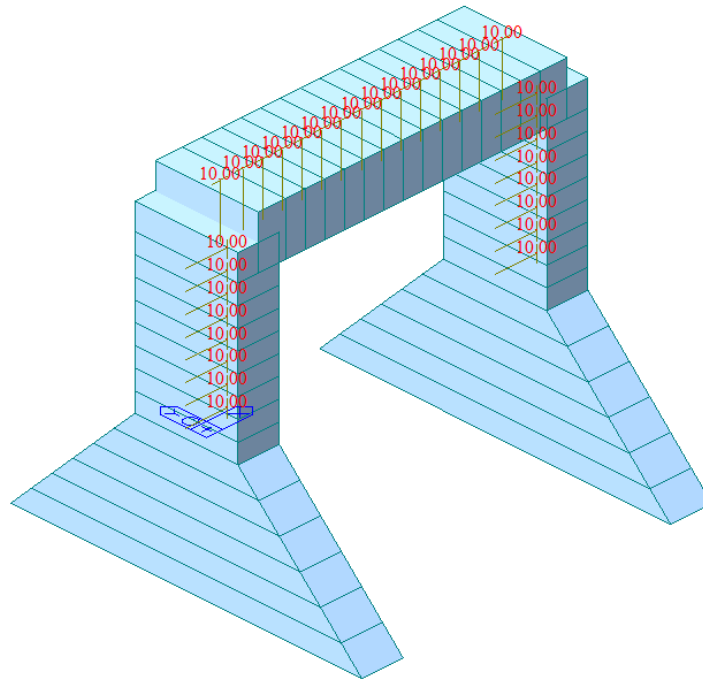
Figura 19 – Gradiente termico \Delta T = +10\text{ }^{\circ}\text{C}
