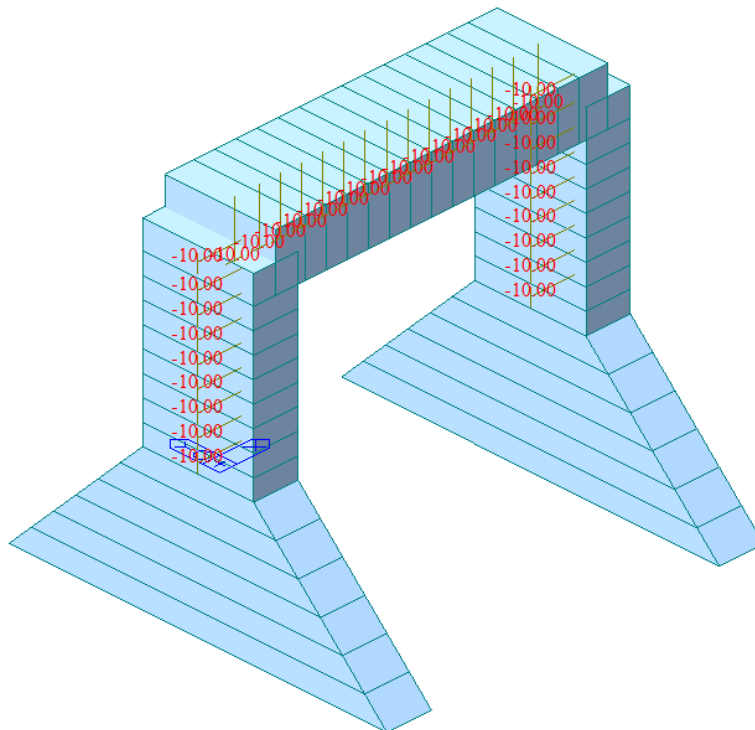
Figura 20 – Gradiente termico \Delta T = -10\text{ }^{\circ}\text{C}
