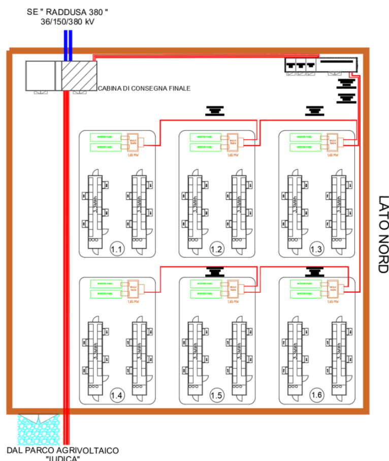
FIGURA 3: LAYOUT BATTERY PACK
