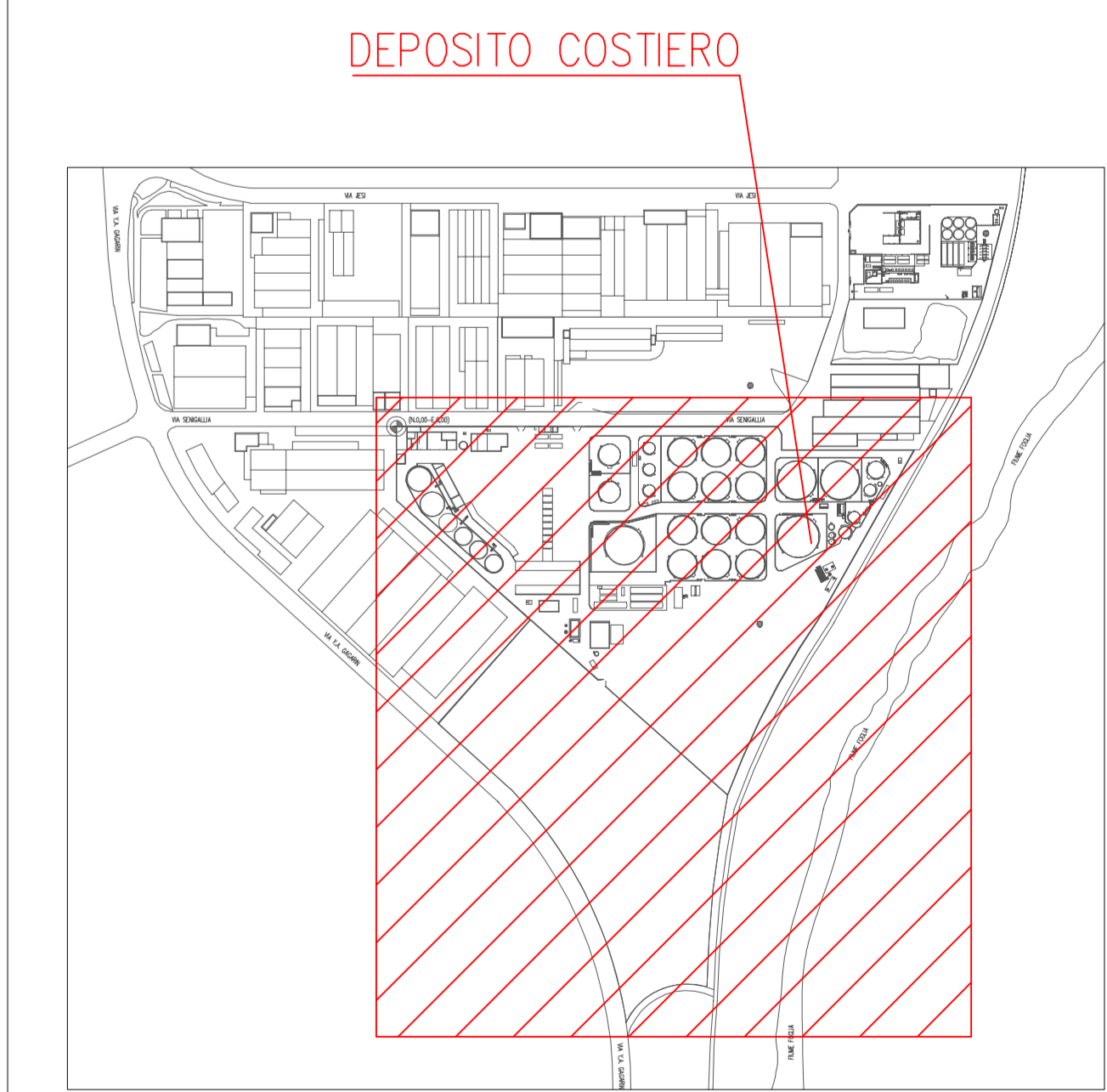
KEY PLAN - AREA FOX PETROLI
