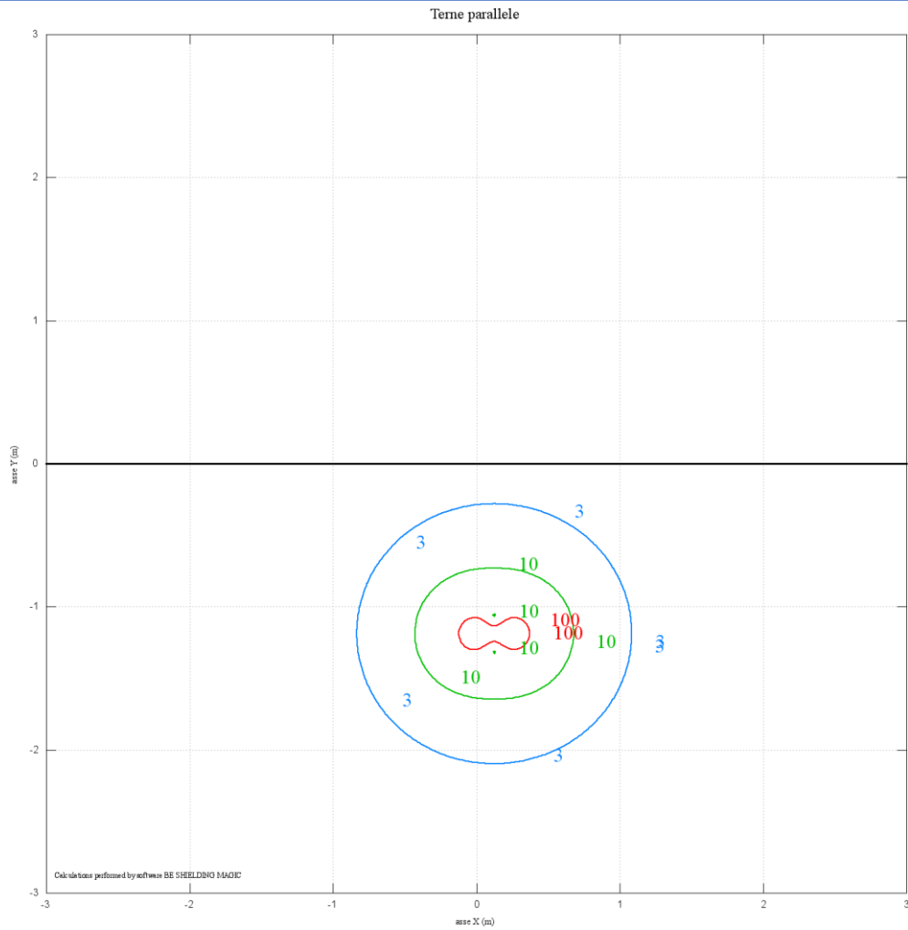
Figura 13: Anello SPS, 2 terne, curve isolivello
