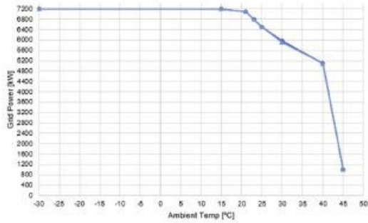
Temperature De-rate Curve – Standard Cooler Top
