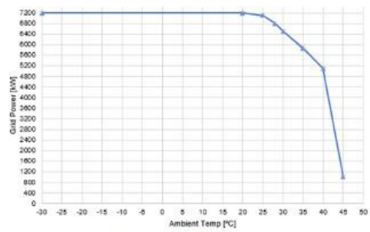
Temperature De-rate Curve – (Optional) Cooler Top
