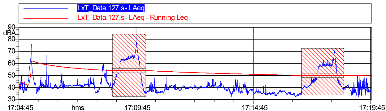
Time history
