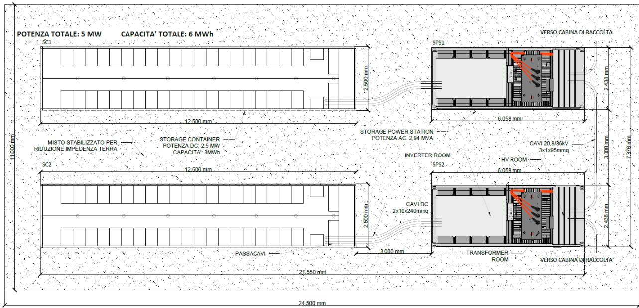
Figura 5: Dettaglio storage container e storage power station
