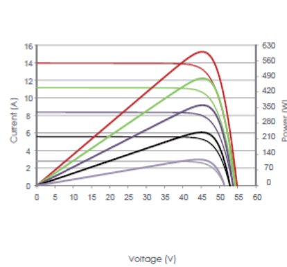
Current-Voltage & Power-Voltage Curves (600W)
