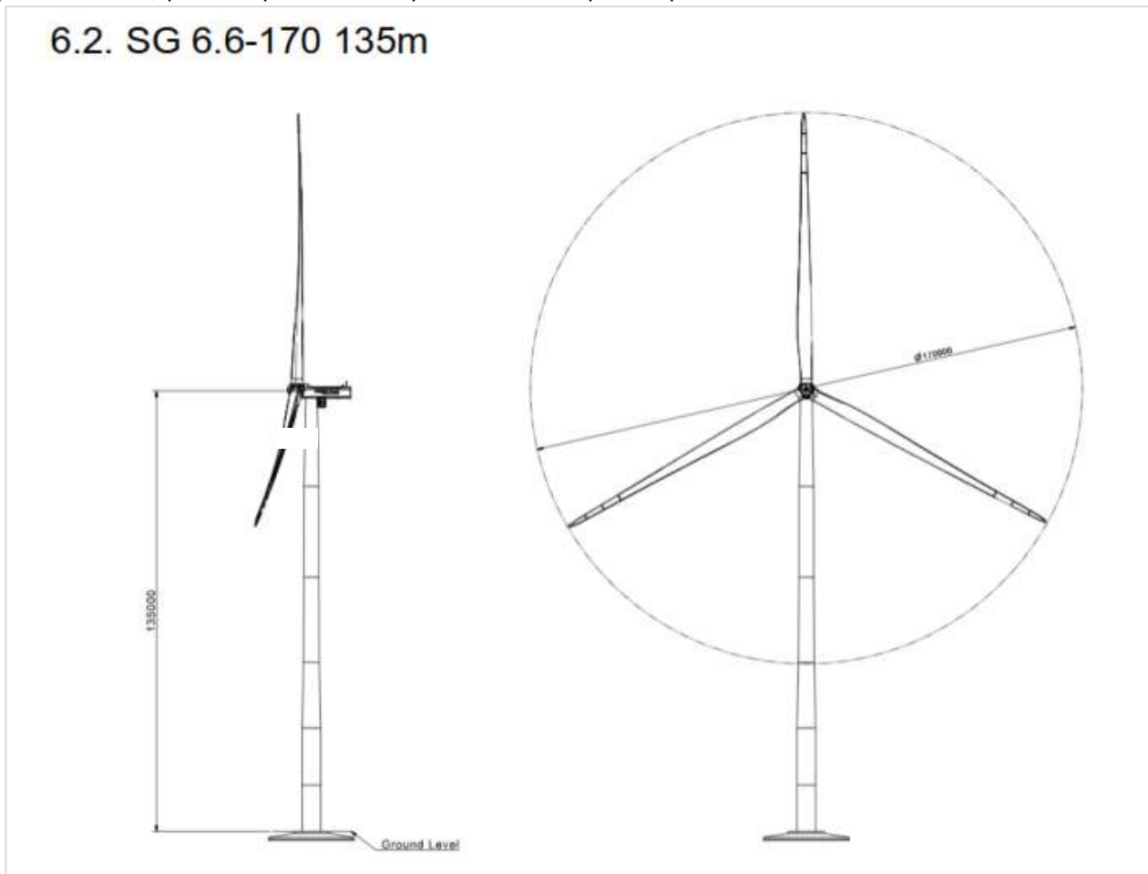
Figura 1_Layout turbina SG 6.6-170
