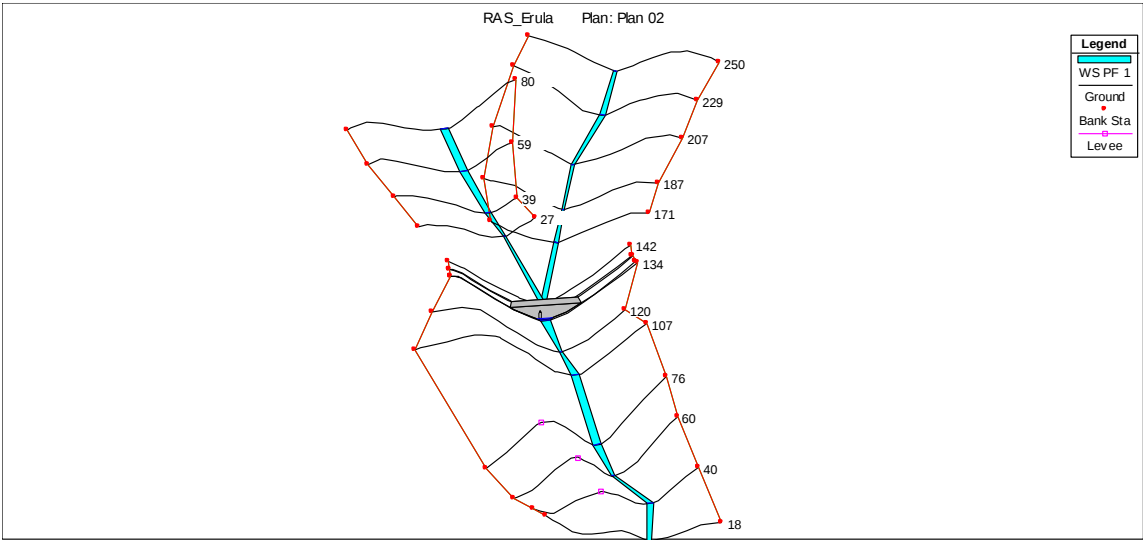
Rappresentazione 3D – River 2 – River 3 – River 2 – Lower (Bacino 2)
