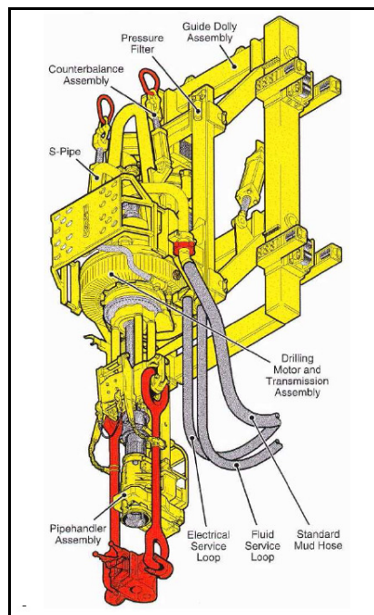
Figura 3-16: Top Drive System
