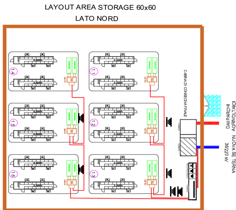
FIGURA 4: LAYOUT BATTERY PACK
