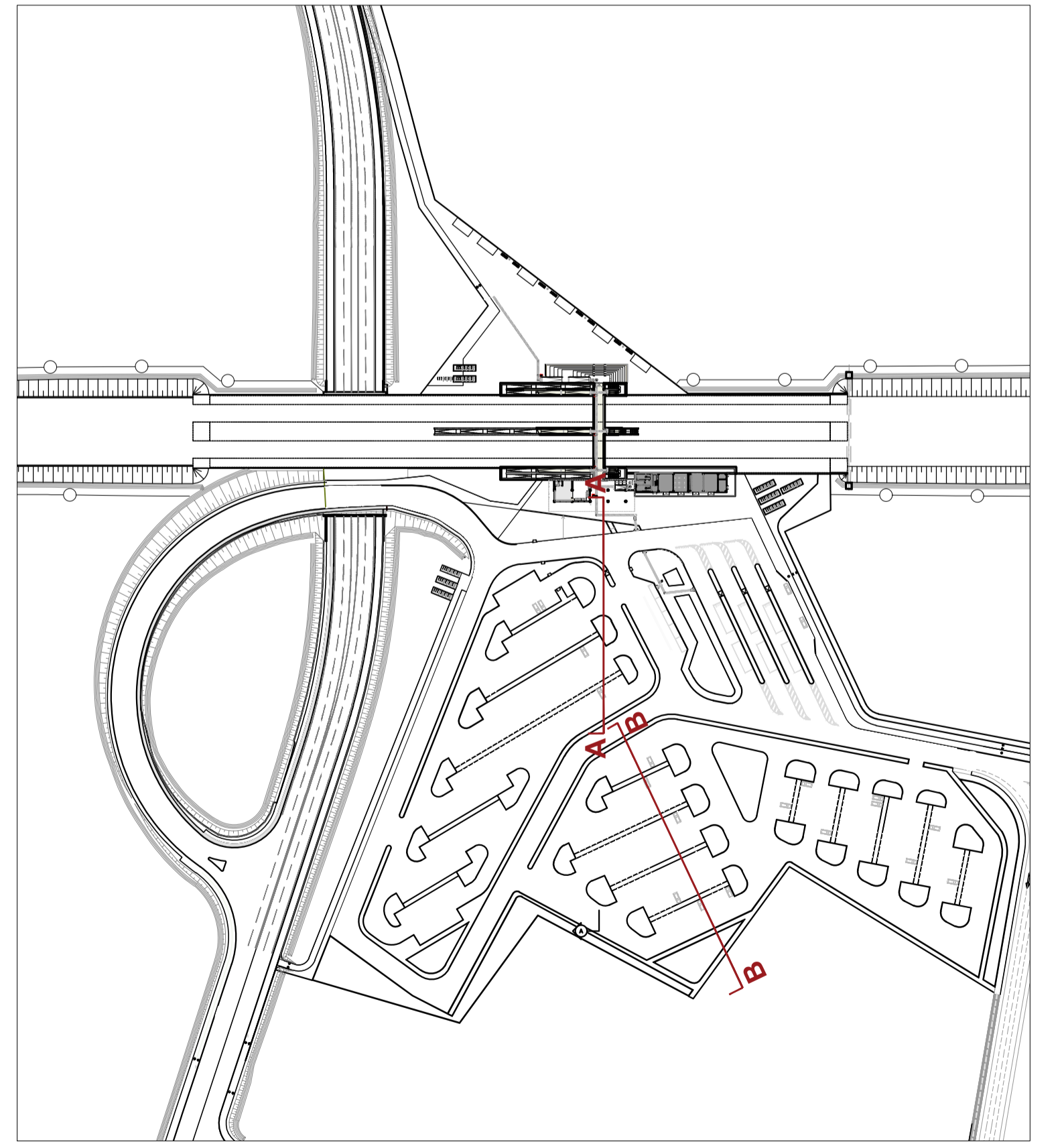
KEY PLAN
