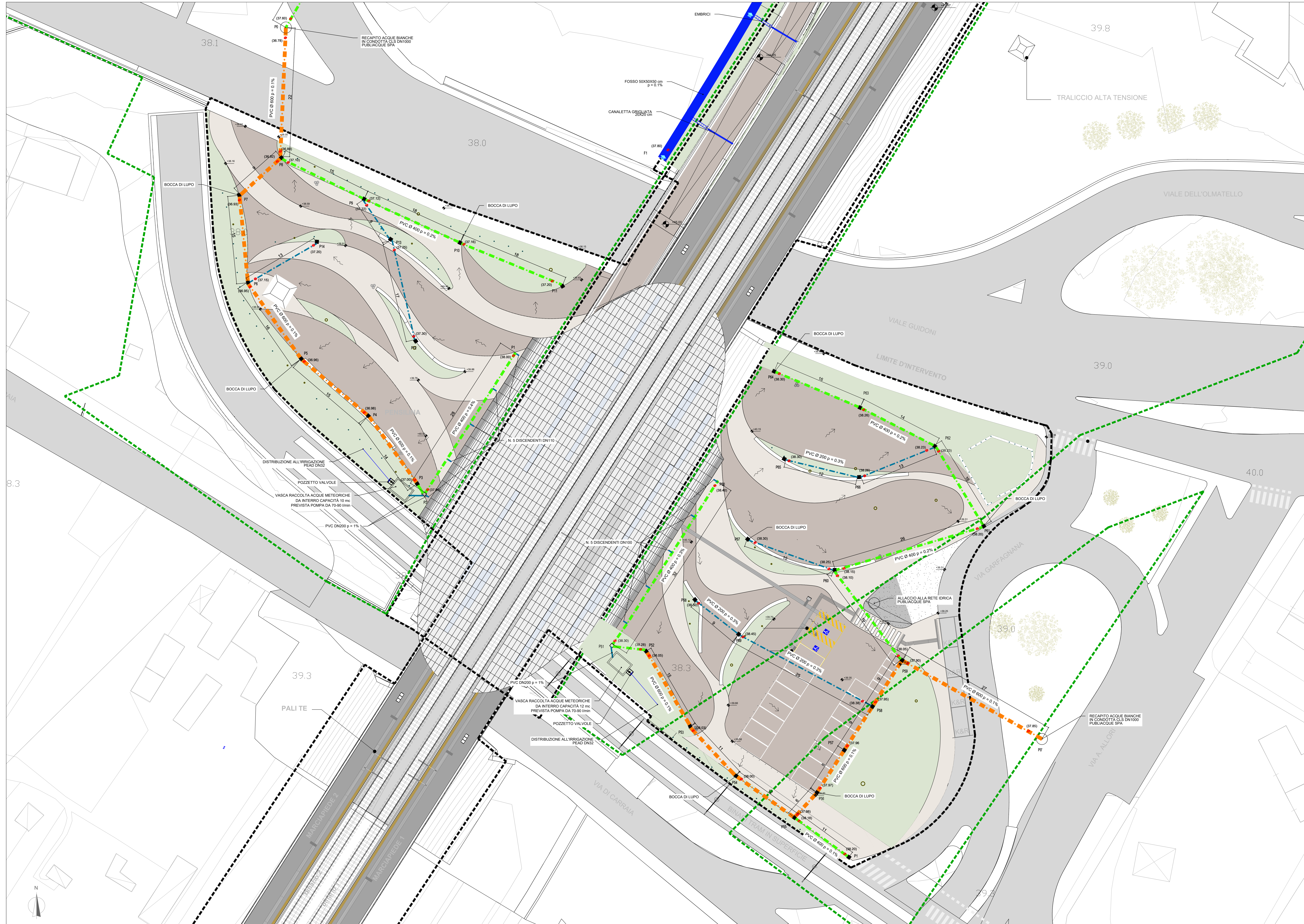
PLANIMETRIA AREE ESTERNE 1 : 200
