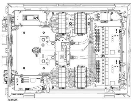
Figura 10: Combiner box
