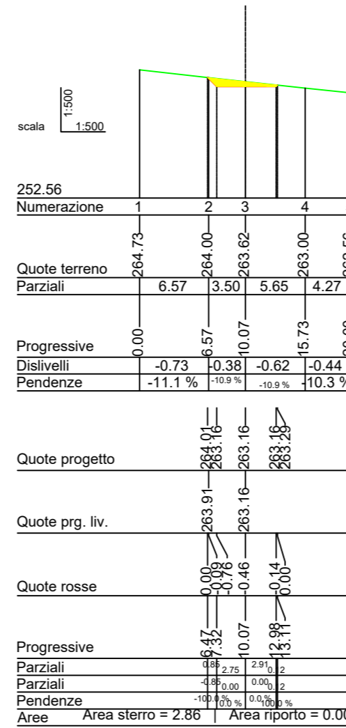
Sez_32 Prog.=635.752
