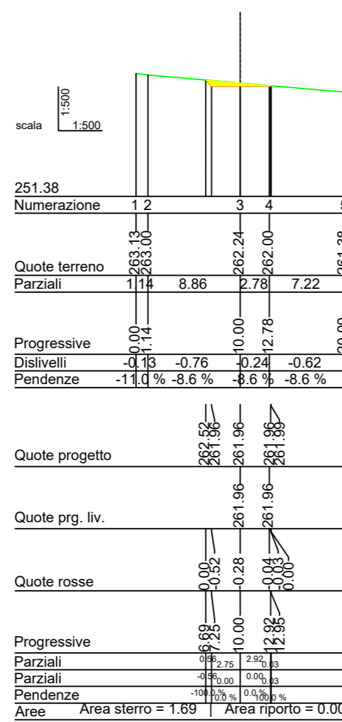
Sez_30 Prog.=595.752
