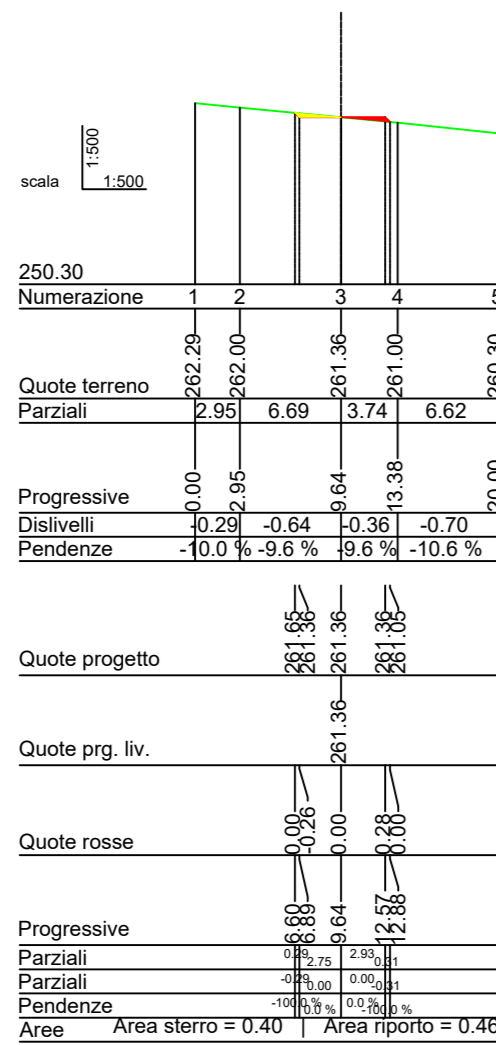
Sez_29 Prog.=575.755
