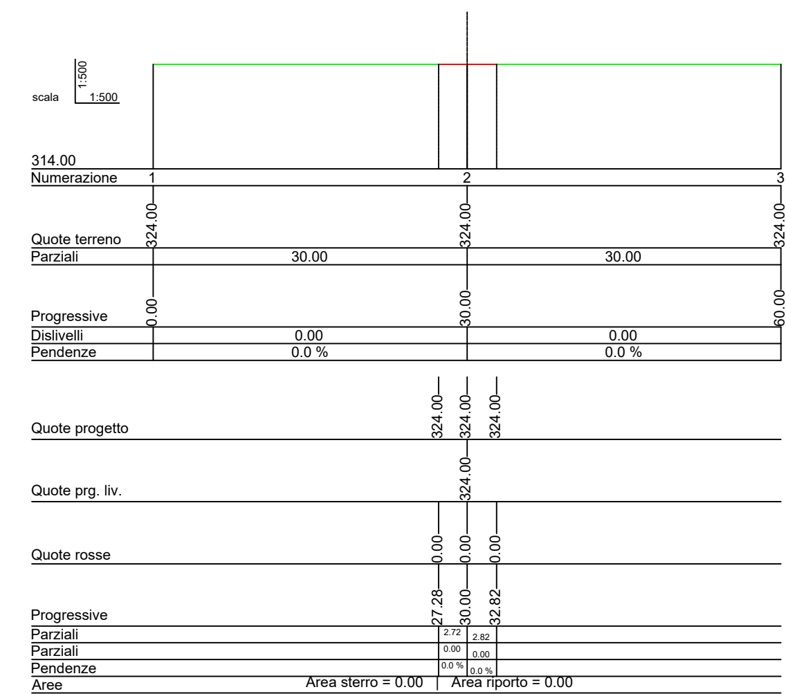
Sez_19 Prog.=353.533
