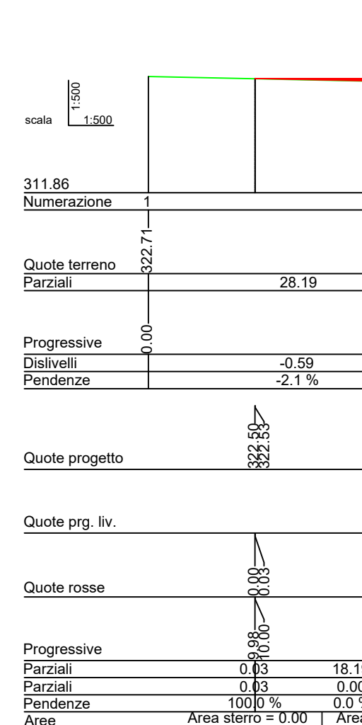
Sez_22 Prog.=416.280
