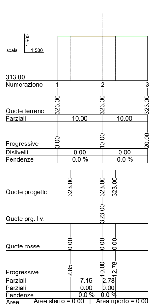
Sez_21 Prog.=393.533
