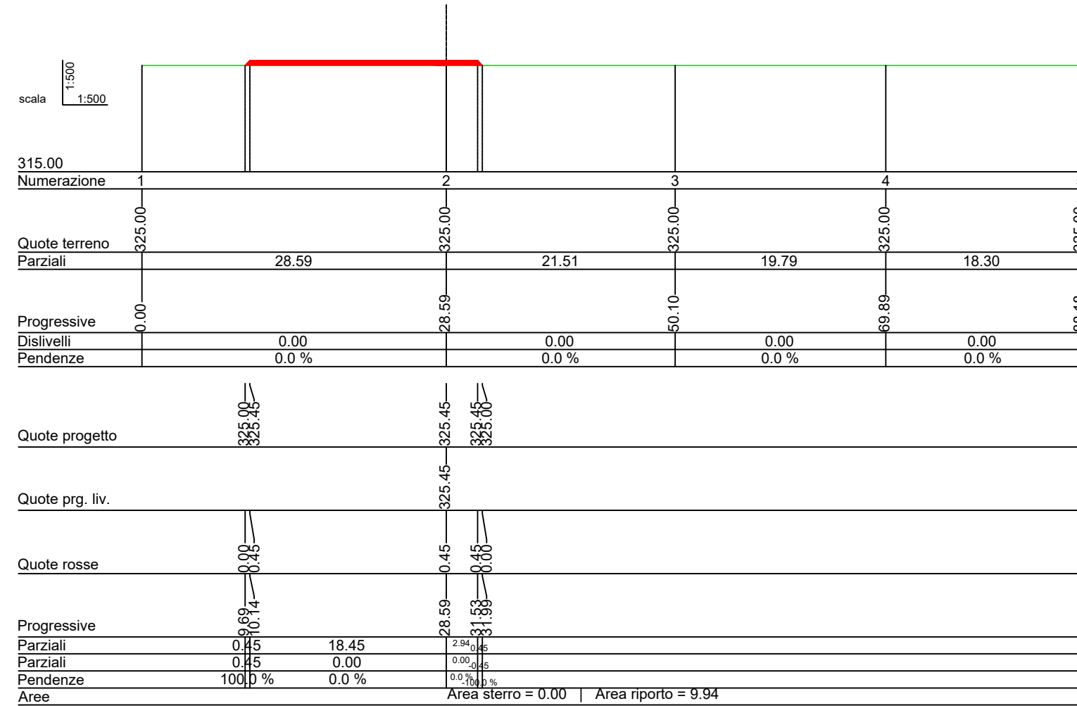
Sez_13 Prog.=233.533
