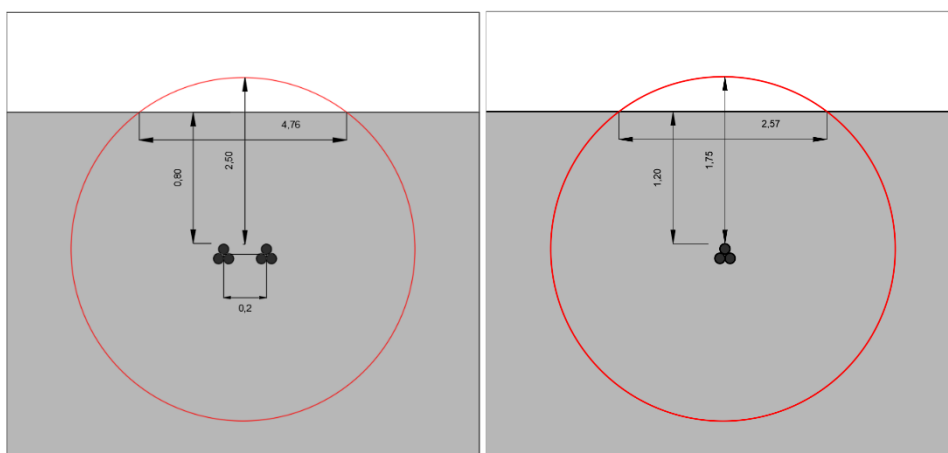
Cavi ARG7H1E(X) 18/30 kV 185 mm 2
