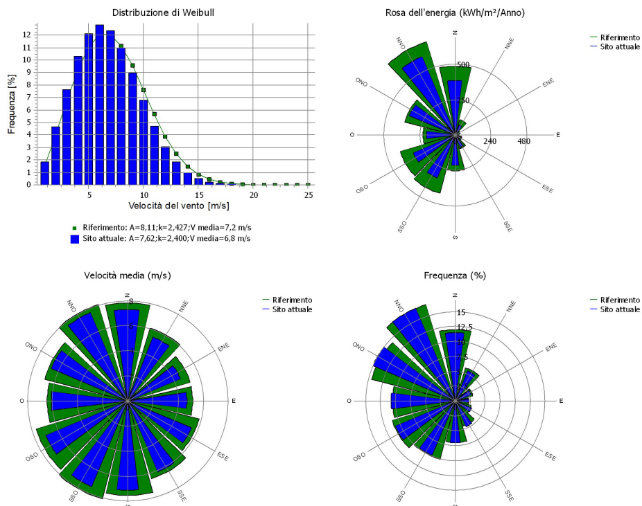
Figura A – Wind Frequency Rose
