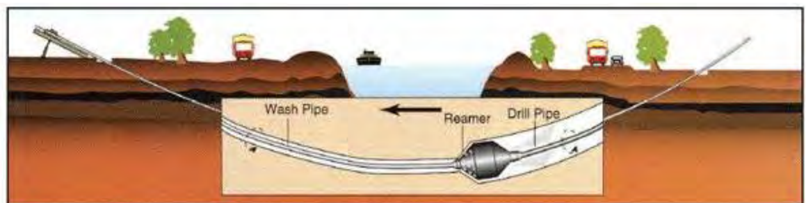
PRE-REAMING
