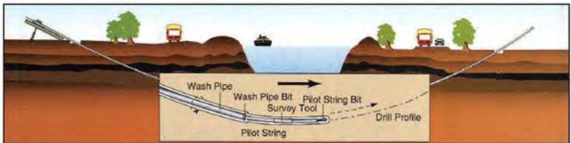
PILOT HOLE
