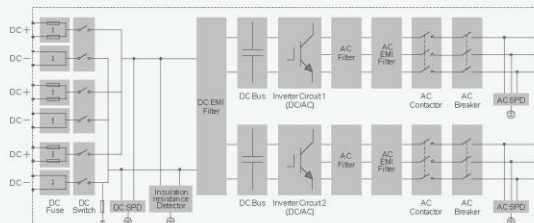
Circuit Diagram
