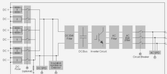
Circuit Diagram
