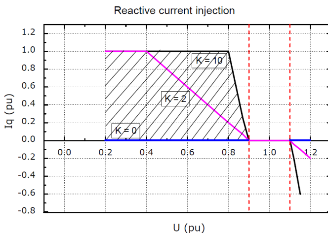
Figure 7: Reactive current injection
