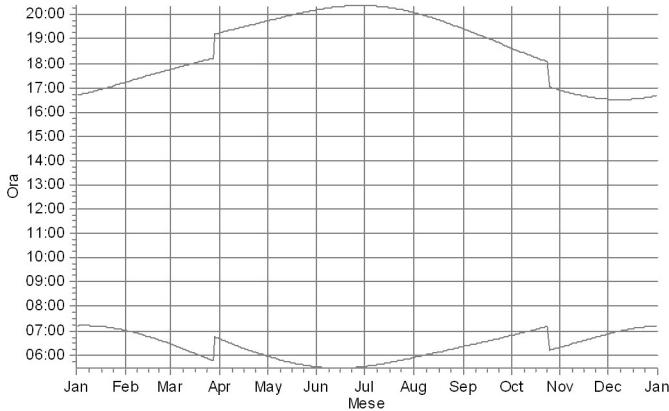
3: Siemens Gamesa SG 6.0-170 6200 170.0 !O! hub: 135,0 m (TOT: 220,0 m)
