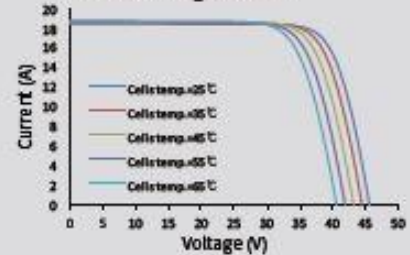
Current-Voltage (660W)
