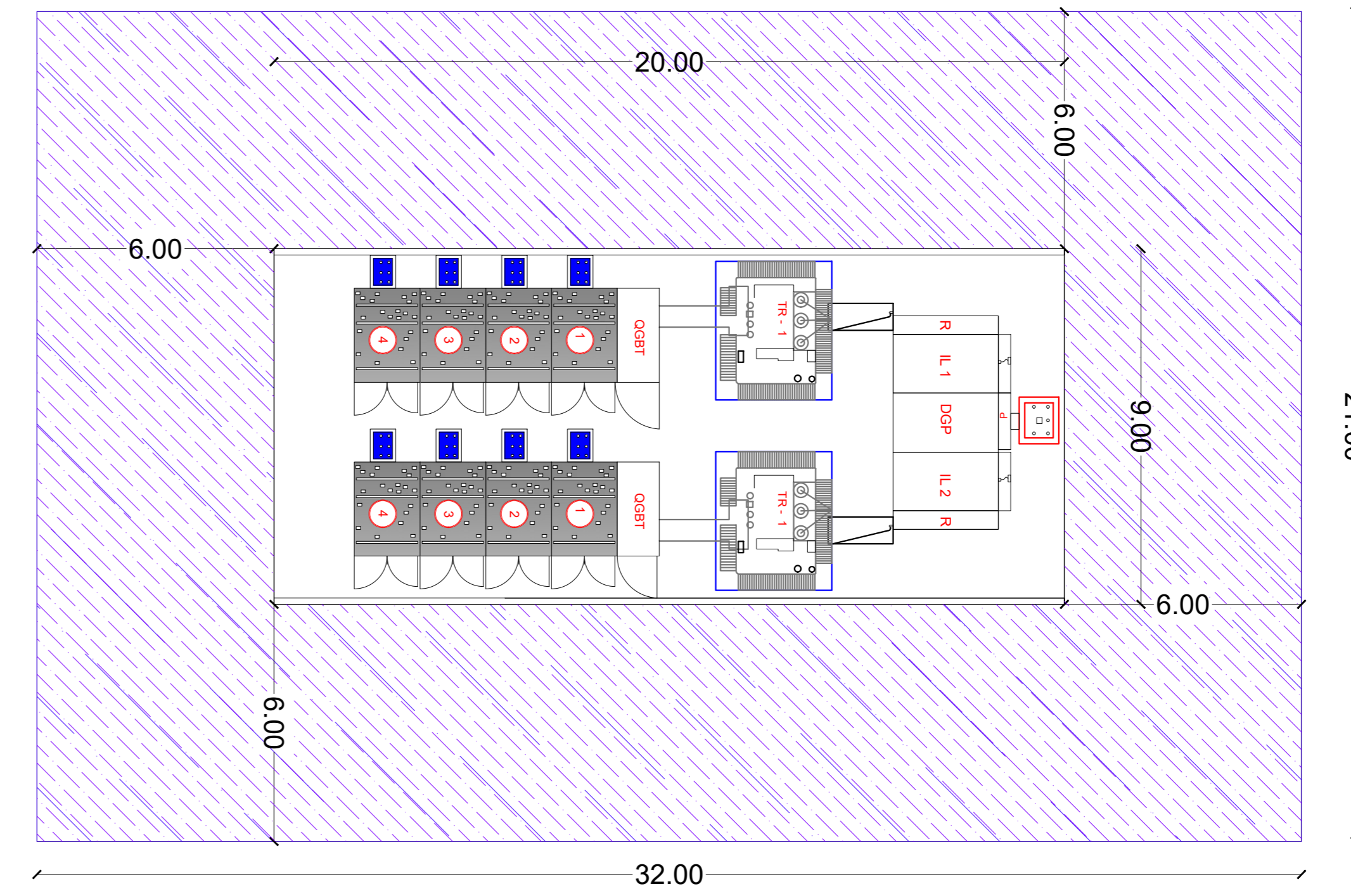
D.P.A - POWER STATION SCALA 1:100
