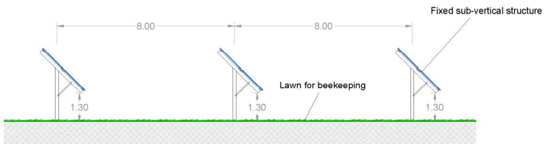
Plot 2 agro-photovoltaic type section
