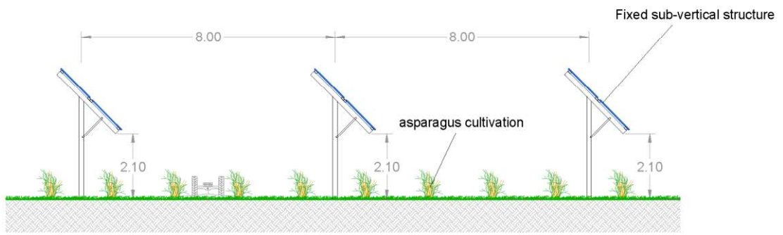
Plot 1 agro-photovoltaic type section
