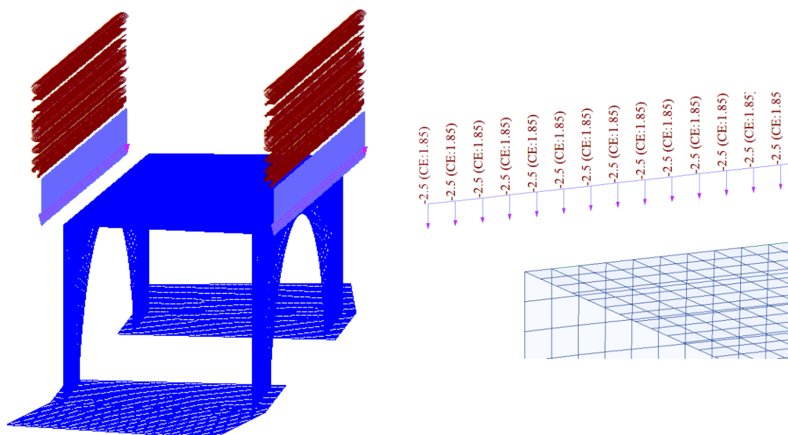
Figura 21: Carichi velette
