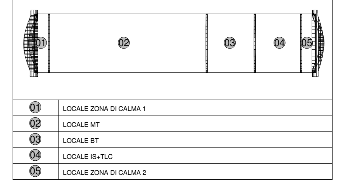
KEY MAP BYPASS PPT 48-932
