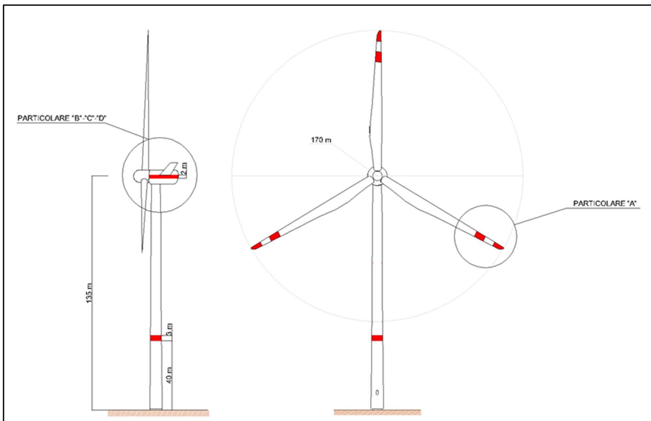
Figura 6.1.1: Profilo aerogeneratore SG170 – 6,0 MWp – HH = 135 m – D = 170 m
