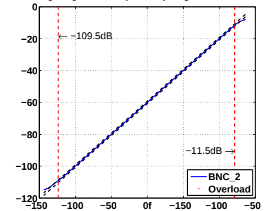
Level Linearity Test at 15.849Hz for Channel BNC_2 C-weighting Gain 0dB passed (Range: 98dB Tol.: 70dB)
