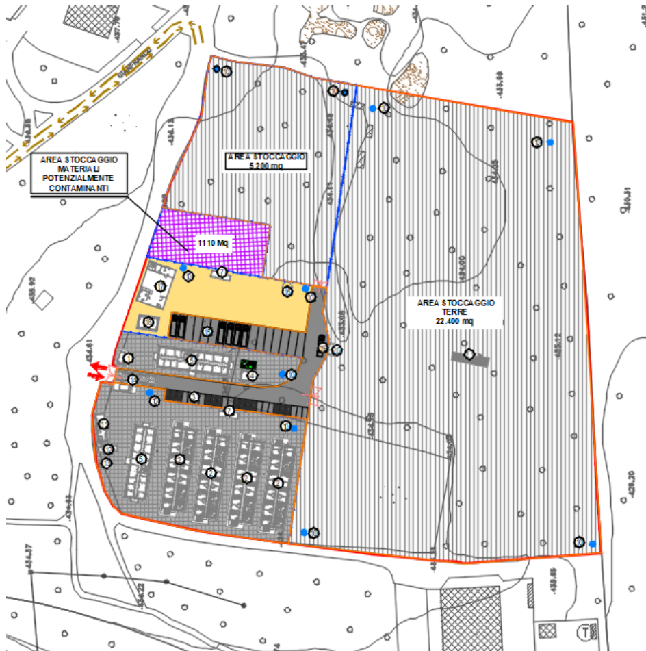
Layout del Campo base CB02
