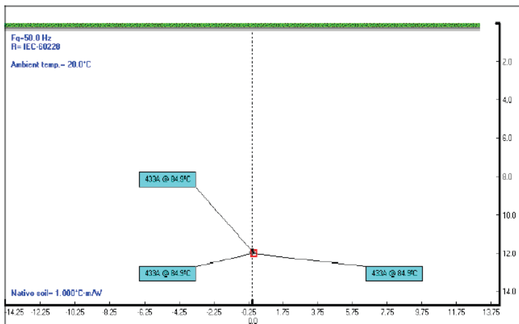
Fig. 1. One circuit in trefoil formation, HDD at depth 12 m. Single point bonding. The ampacity is 433 A at 85°C.
