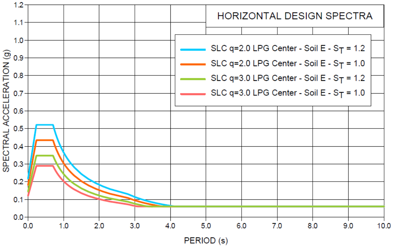
Figure 6-4 - Horizontal Design Spectra for SLC Limit State – Example of Class IV
