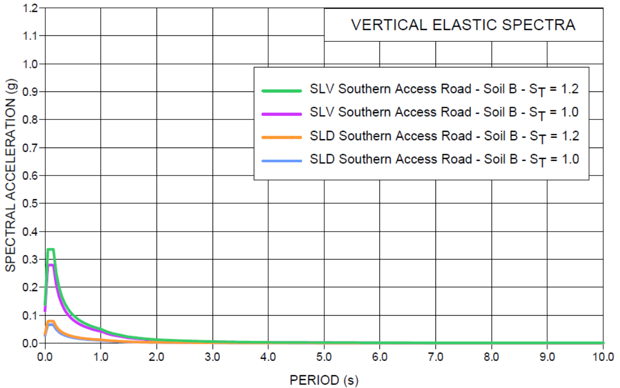
Figure 6-6 - Vertical Elastic Spectra – Example of Class III
