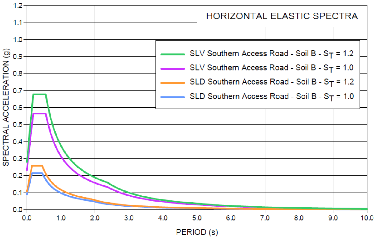
Figure 6-2 - Horizontal Elastic Spectra – Example of Class III
