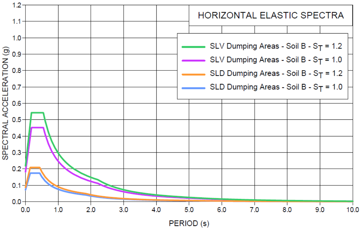
Figure 6-1 - Horizontal Elastic Spectra – Example of Class II
