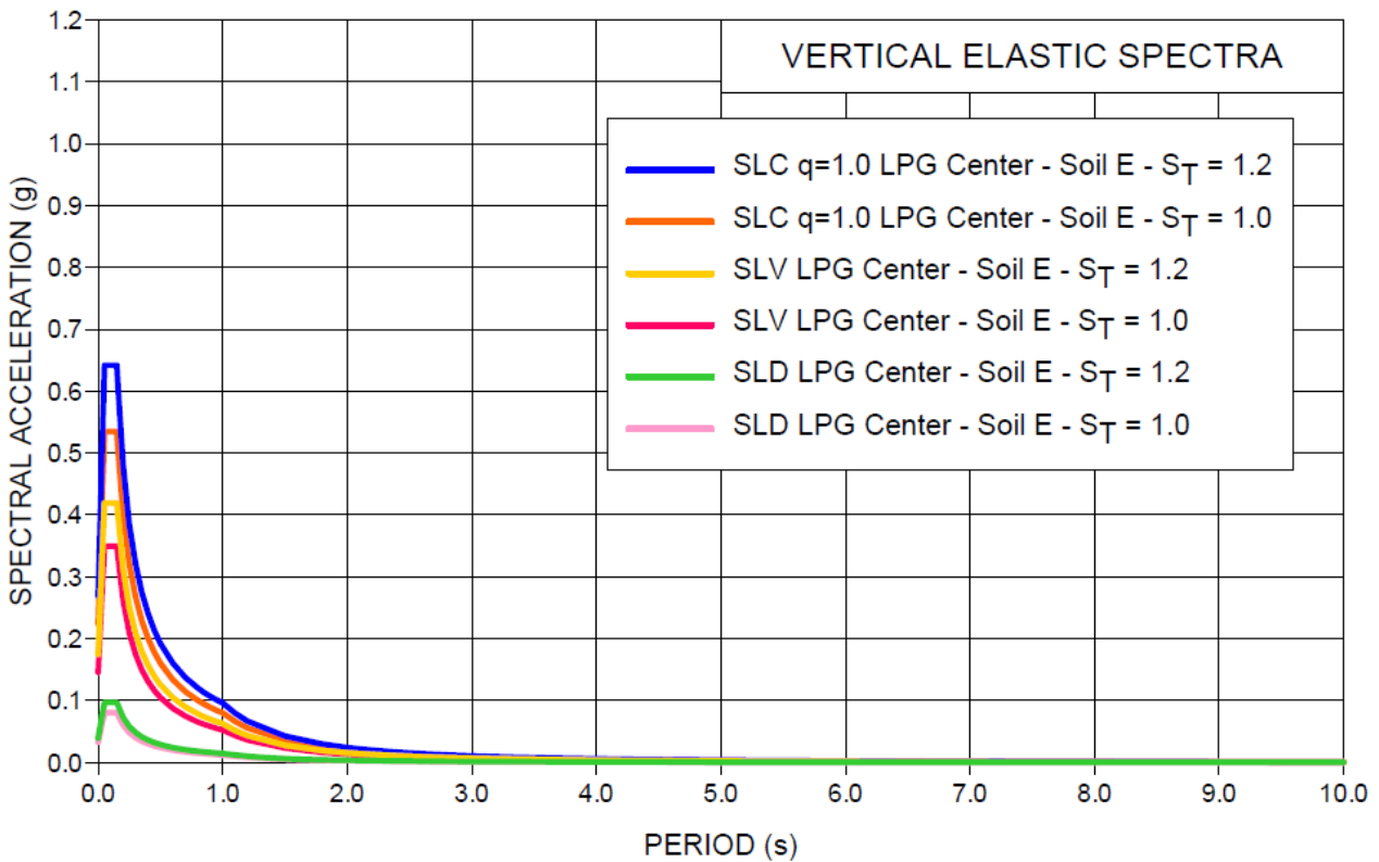
Figure 6-7 - Vertical Elastic Spectra – Example of Class IV
