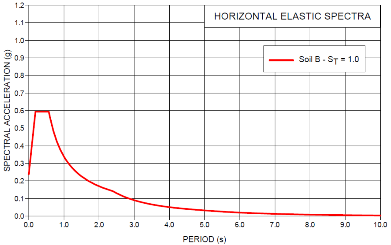
Figure B-1 - Elastic Horizontal Spectra for 5% Damped Horizontal Ground Motion Main Structure in the Oil Center - SLV
