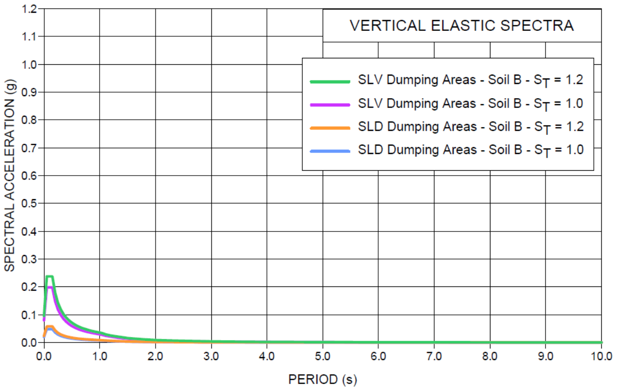
Figure 6-5 - Vertical Elastic Spectra – Example of Class II
