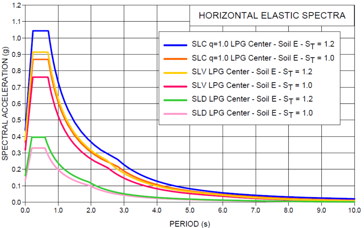
Figure 6-3 - Horizontal Elastic Spectra – Example of Class IV
