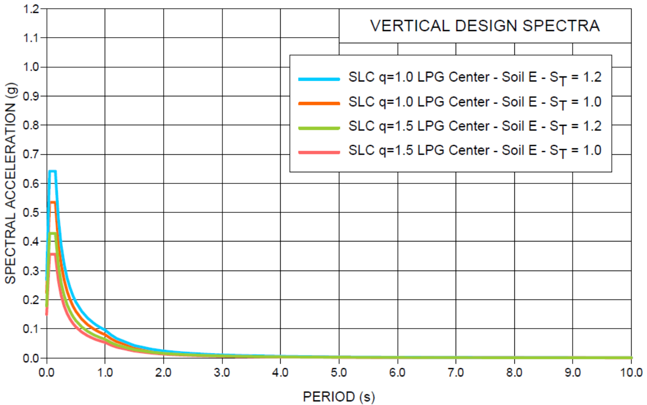
Figure 6-8 - Vertical Design Spectra for SLC Limit State – Example of Class IV
