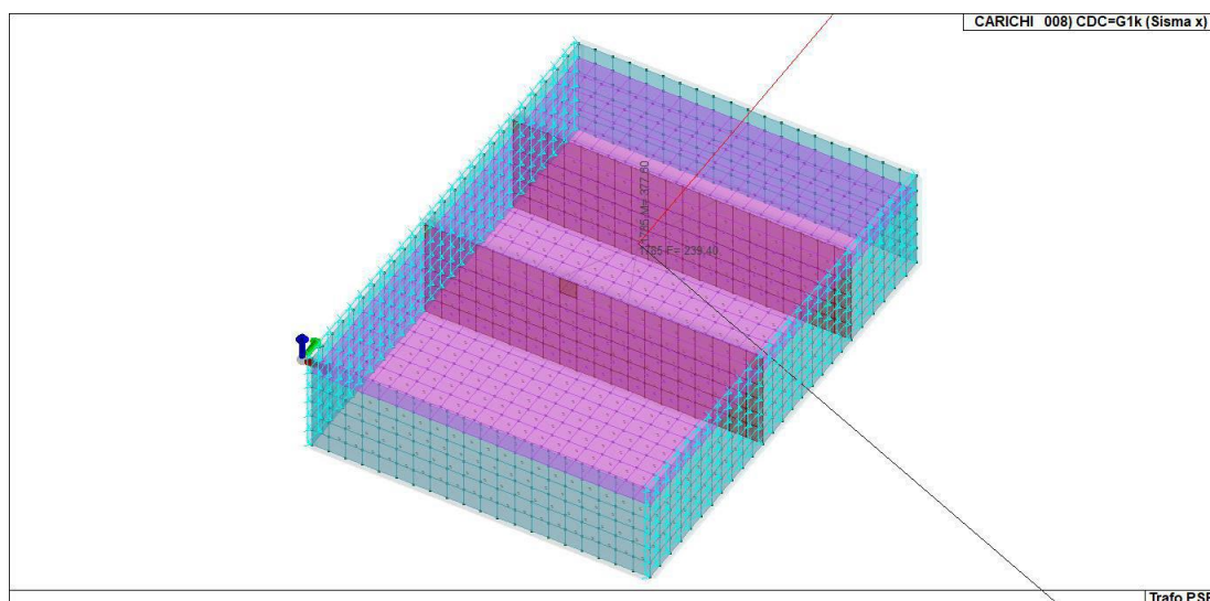
Figura 11-8 CDC_008_CDC=G1k (Sisma x)
