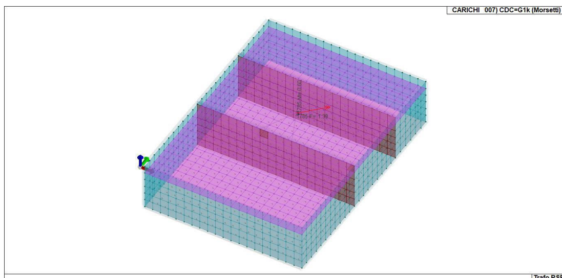
Figura 11-7 CDC_007_CDC=G1k (Morsetti)
