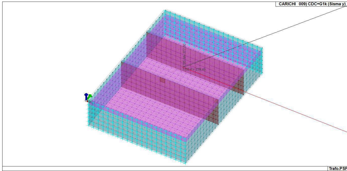
Figura 11-9 CDC_009_CDC=G1k (Sisma y)
