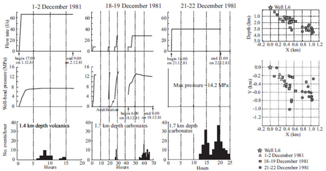
(a) Latera Well L6 injection records and recorded microseismicity (b) Hypocentre locations
