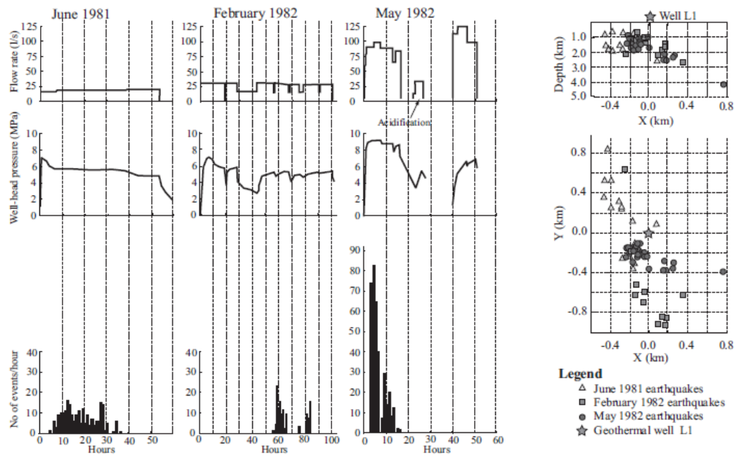
(a) Latera Well L1 injection records and recorded microseismicity (b) Hypocentre locations
